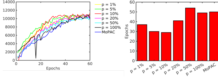
Figure 3: Ablation study for elite percentage: Reward performance curve (left) and Acceleration analysis as epochs to reach 10000 rewards (right)
