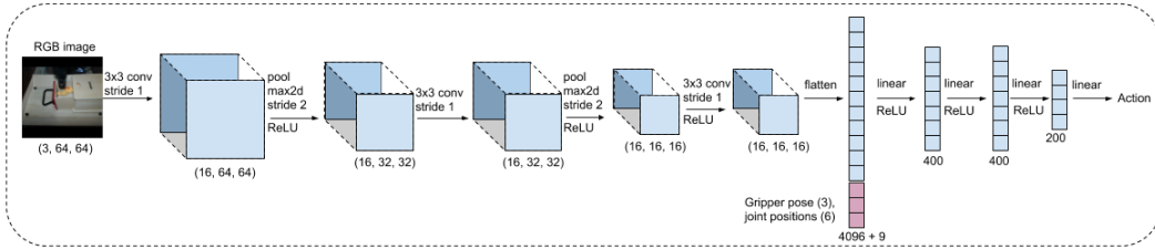
Figure 7: Neural network architecture for real robot experiments. Here we show the architecture for the policy network for real robot experiments. The Q-function architecture is identical, except it also has the action as an input that is passed in after the flattening step. We map high dimensional image observations to low level robot commands, i.e. desired position of the end-effector, and gripper opening/closing.
