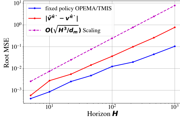
Figure 3: Log-log plot showing the dependence on horizon of uniform OPE and pointwise OPE via learning ( |\hat{v}^* - v^{\pi^*}| ) over a non-stationary MDP example.
